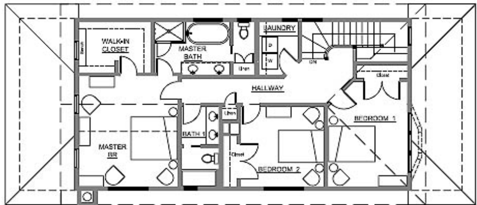
SECOND FLOOR PLAN - NEW
