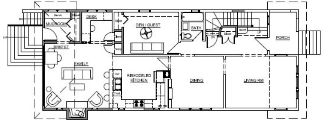
FIRST FLOOR PLAN - NEW
